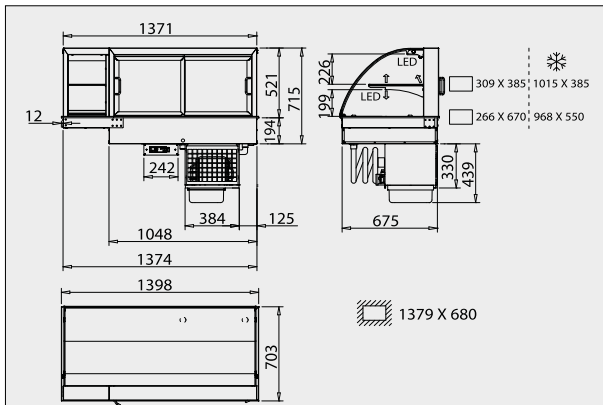
Art.-Nr. 12344 WIHA Snack-Counter 520 KOMBI BE - 3k+1
