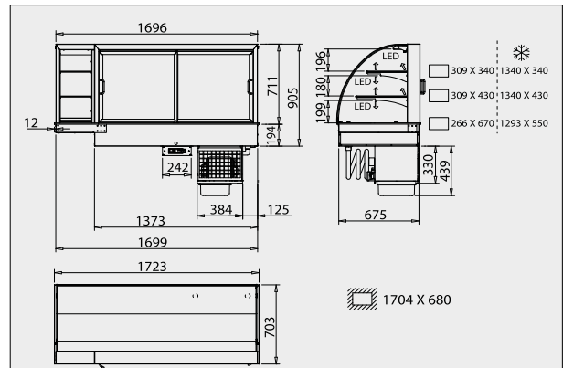
Art.-Nr. 12348 WIHA Snack-Counter 710 KOMBI BE - 4k+1
