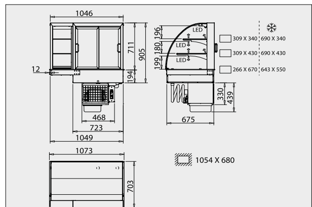
Art.-Nr. 12345 WIHA Snack-Counter 710 KOMBI BE - 2k+1
