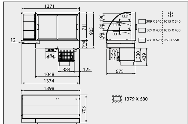
Art.-Nr. 12346 WIHA Snack-Counter 710 KOMBI BE - 3k+1
