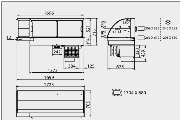
Art.-Nr. 12372 WIHA Snack-Counter 520 KOMBI BE - 4k+1
