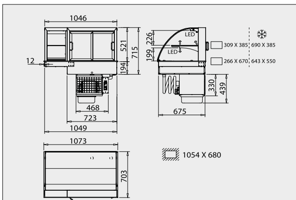
Art.-Nr. 12343 WIHA Snack-Counter 520 KOMBI BE - 2k+1
